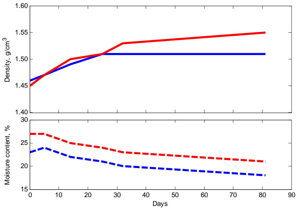
Figure 5 Shrinkage causing an increase in density with moisture content over an 80 day period between March and June 2006. These soils were not rolled during this period. The blue line is for a 26% clay soil and the red line for a 30% clay soil. The higher clay soil (red) has more moisture content but shrinks more so the density is greater.
